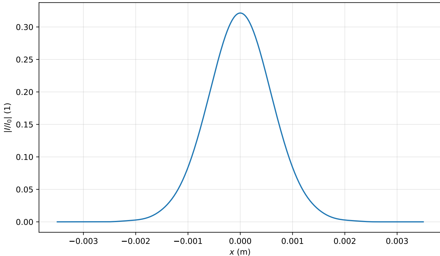
Intensity profile I(x, y = 0, z = 3.662m)/I_0 , P_{in}=0.3P_{cr} , artificial time
